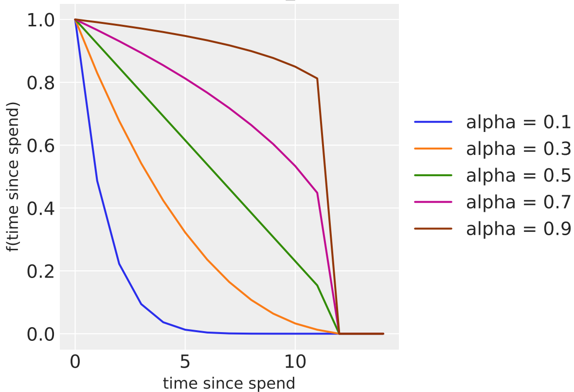
Binomial Adstock with I_{\max} = 12
